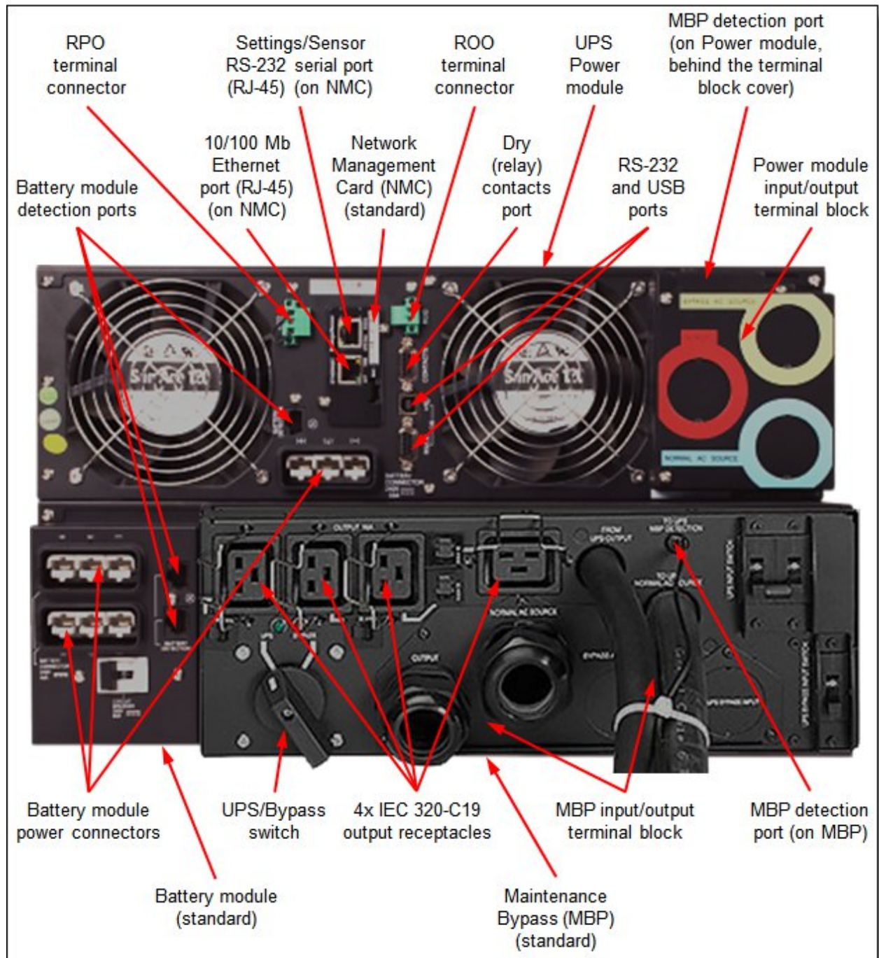
Figure 6. Rear view of the RT8kVA or RT11kVA 6U 3:1 Phase Rack or Tower UPS (380-415VAC)
